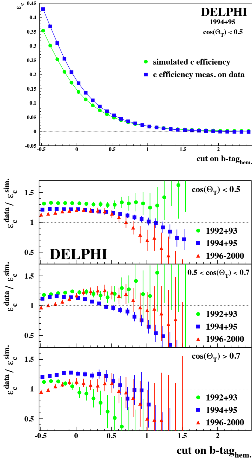
Figure 2: The measured efficiency of c -quark hemispheres, as a function of the cut on b\text{-tag}_{hem} , in simulation compared to real data following the procedure outlined in the text. The upper plots details the situation in the central region for the 1994+95 data, while the triple plot below summarises the agreement found in all three VD set-ups and polar angle ranges.
