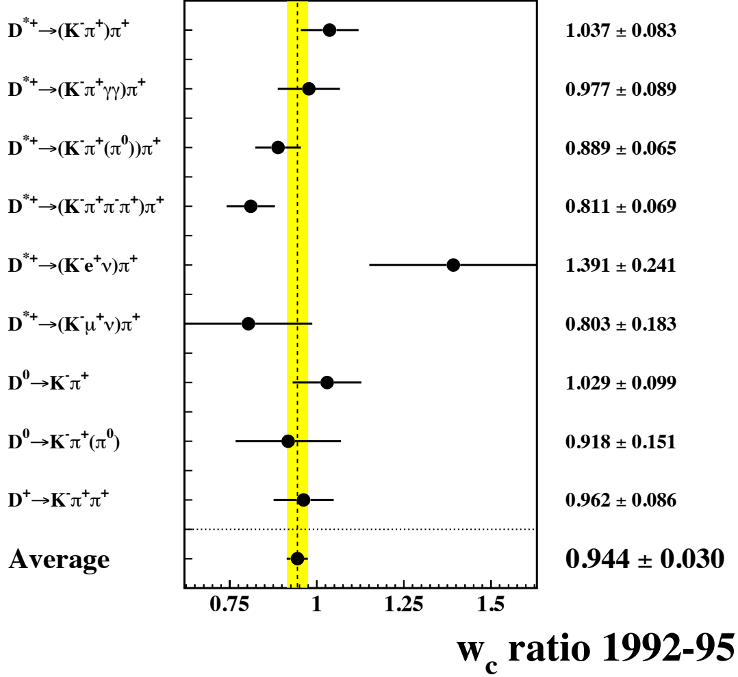
Figure 11: The ratio of real data to simulation in the c quark charge identification w_c provided by a flav_{hem} tag in a hemisphere opposite a reconstructed D . The final result is decomposed in the 9 different decay channels used in [14].
