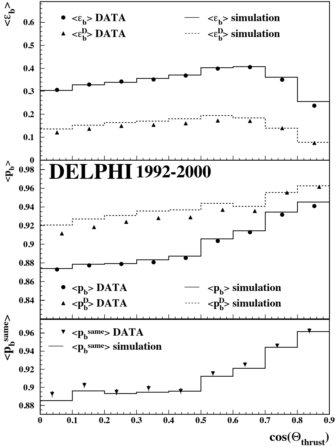
Figure 12: The b efficiencies \epsilon_b and \epsilon_b^D and the purities p_b and p_b^D for single and double unlike-sign tagged events as a function of the polar angle. The purity p_b^{same} for double like-sign tagged events is relevant for measuring the charge tagging probability, w_b^{(D)} .
