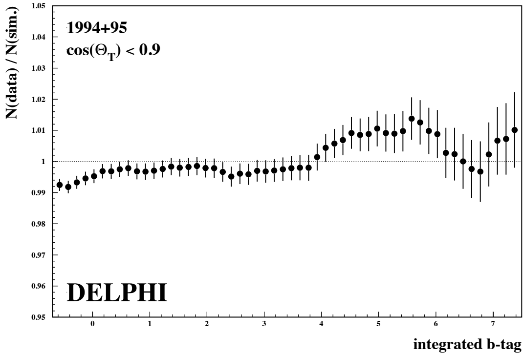
Figure 4: The (integrated) b-tag ratio of real to simulated events after application of the correction functions to simulated b and c quark events. The data is from the 1994+95 DELPHI data set. Different correction functions for the \cos\theta_{\bar{F}} intervals of [0.0, 0.5) , [0.5, 0.7) and \geq 0.7 were applied before integrating over the full polar angle.
