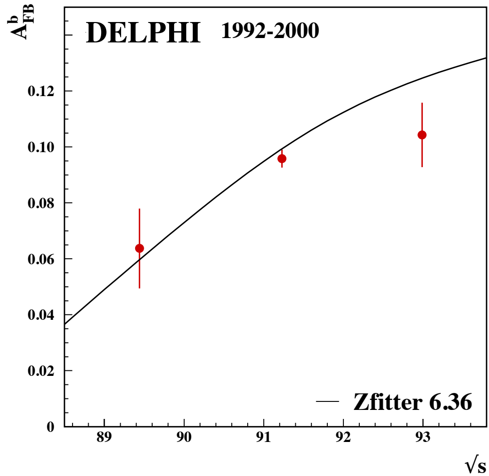
Figure 18: The A_{FB}^b results versus the centre-of-mass energy. The line represents the Standard Model prediction obtained from ZFITTER (see text for details).
