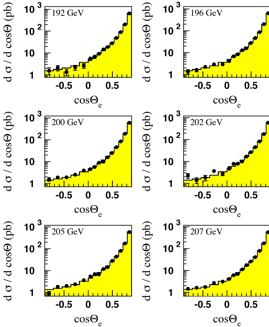
Figure 1: LEP averaged differential cross-sections for e^+e^- \rightarrow e^+e^- at energies of 192–207 GeV. The SM predictions, shown as solid histograms, are computed with BHWIDE [2].
